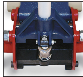
Angular Pump Piston Feature
